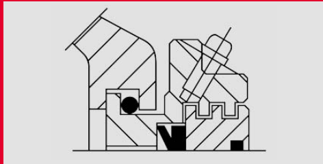
TACK Seals
